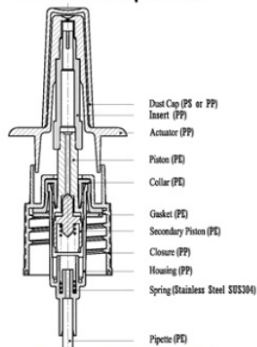
Drawing for XJT sprayers No POM components
